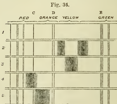
1. Solar Spectrum. 2. Oxidized Hæmaglobin. 3. Reduced hæmaglobin. 4. Hæmaglobin decomposed by acids. 5. Hæmaglobin decomposed by alkalies.
